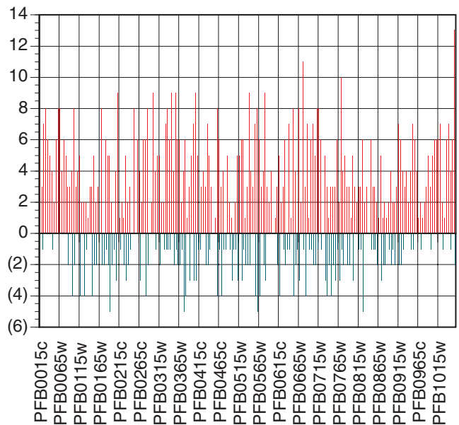
Fig. 6. Demonstration that detection of low-complexity regions by CAST stems from local complexity and not global composition bias. On the x-axis, the 210 open reading frames of P. falciparum chromosome 2 are listed (labels every ten ORFs). On the y-axis, the number of amino acid residue types detected by CAST only (red bars) or by both CAST and a global bias (counts in parentheses, dark green bars). Maximum number of residue types is 20. Significant global composition bias per residue was obtained for all ORFs, by comparing the observed residue composition of each ORF with the average residue composition of Swiss-Prot, Release 38: a chi-square test at 99.5% confidence level with 19 degrees of freedom (chi-square value = 38.6) was used.
